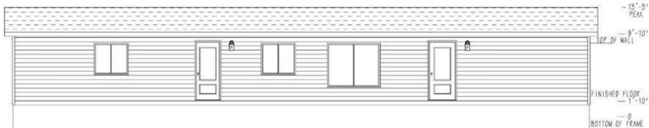
CURBSIDE ELEVATION SCALE: 3/16"=1'-0"
