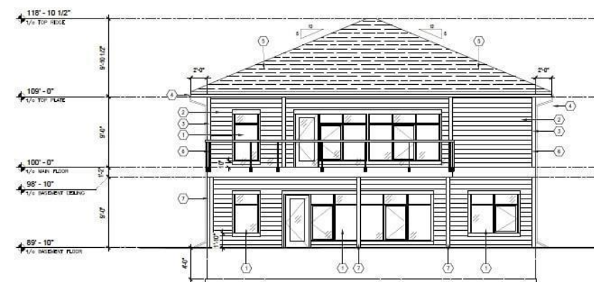
3 SOUTH ELEVATION A3.1 3/16" = 1'-0"
