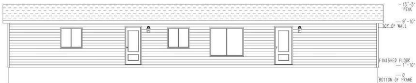
CURBSIDE ELEVATION SCALE: 3/16"=1'-0"
