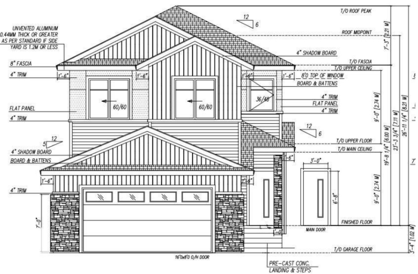
FRONT ELEVATION
