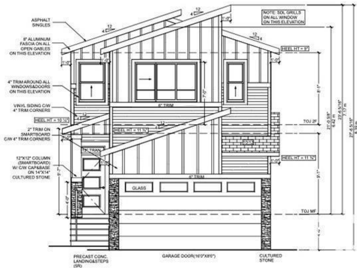
FRONT ELEVATION
