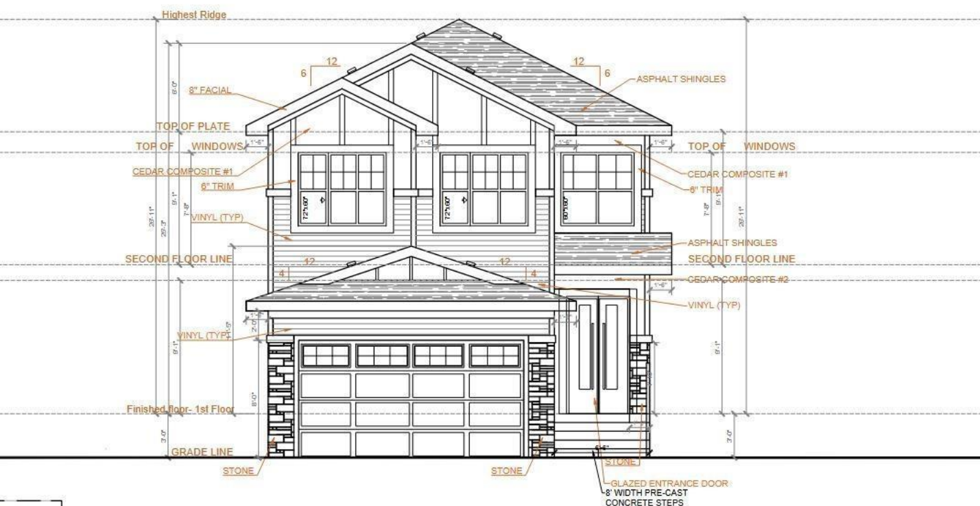
FRONT ELEVATION CRAFTSMAN DESIGN STYLE
