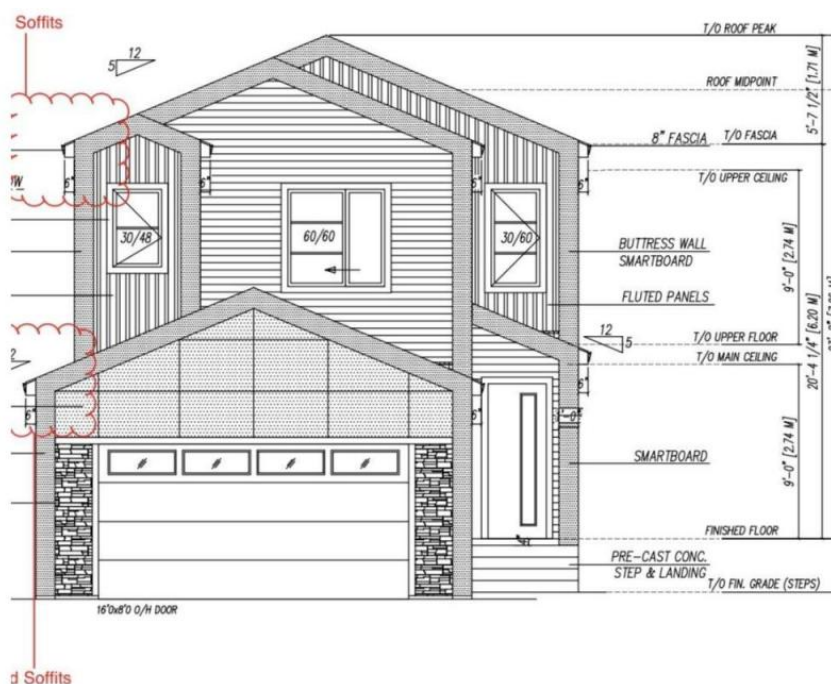
FRONT ELEVATION
