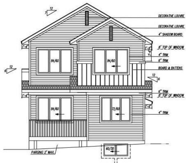
REAR ELEVATION
