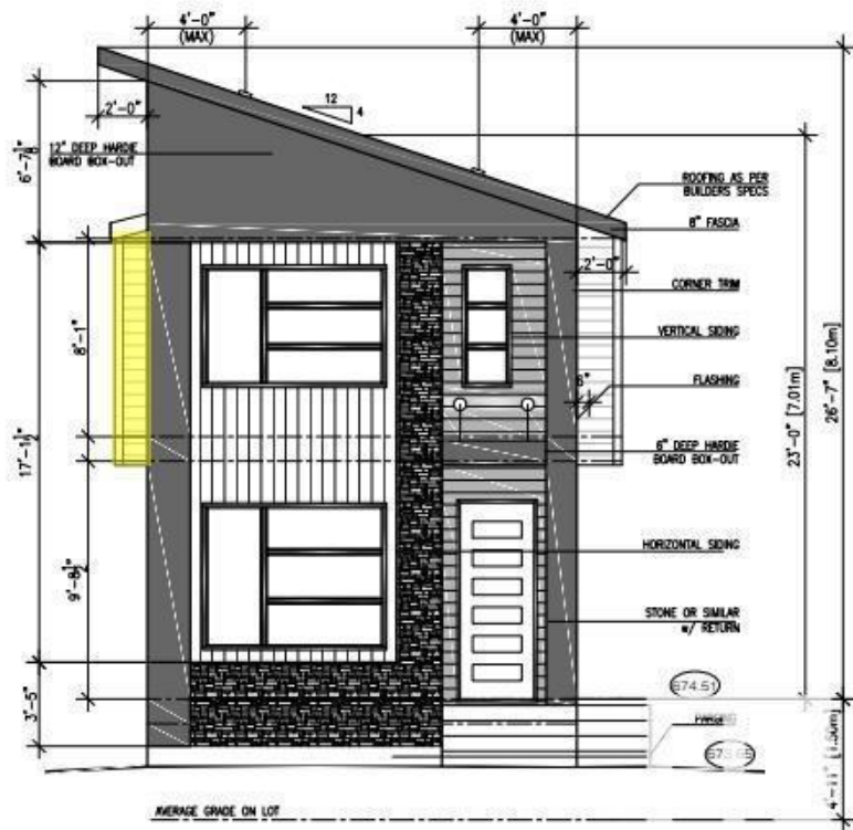
FRONT ELEVATION (LOT 22A) SCALE: 3/16" = 1'-0"
