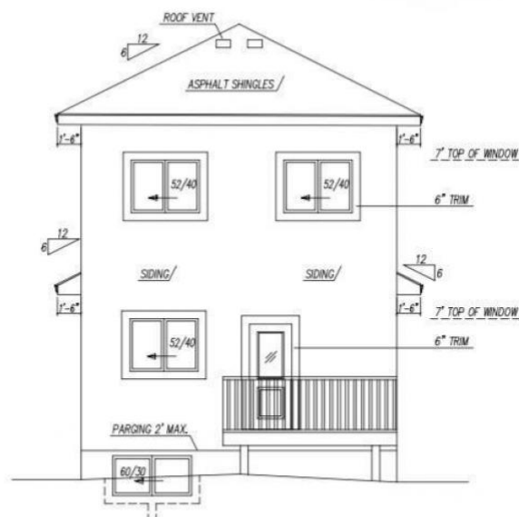
REAR ELEVATION
