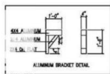
ALUMINUM BRACKET DETAIL
