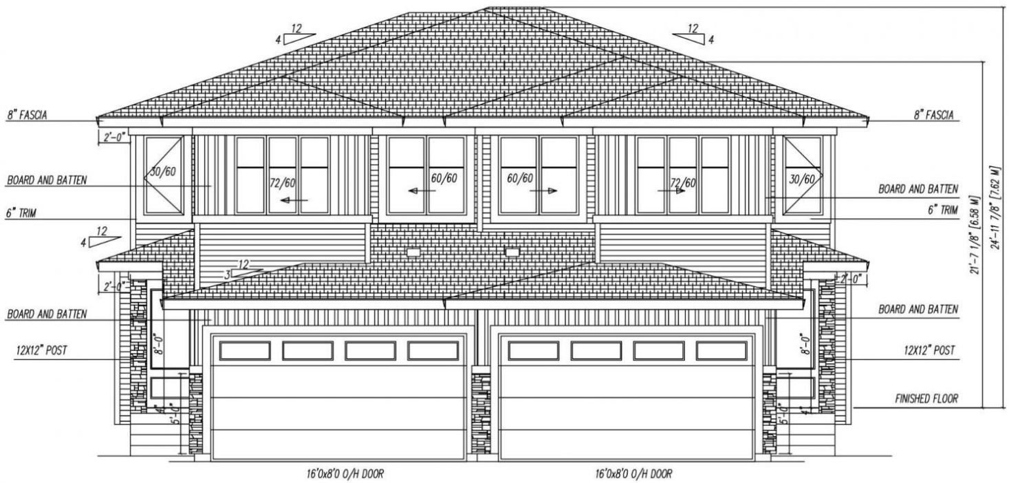
FRONT ELEVATION
