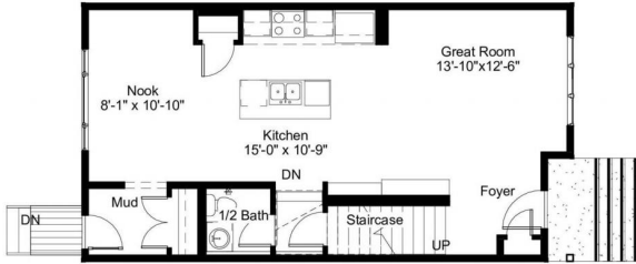
Main Floor Plan 744 SQFT 9'-1" Main Floor Ceiling
