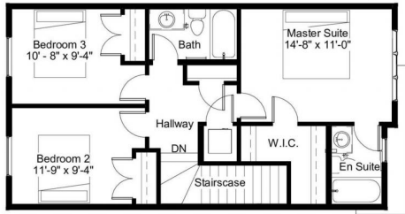
Second Floor Plan 744 SQFT 8'-1" Second Floor Ceiling
