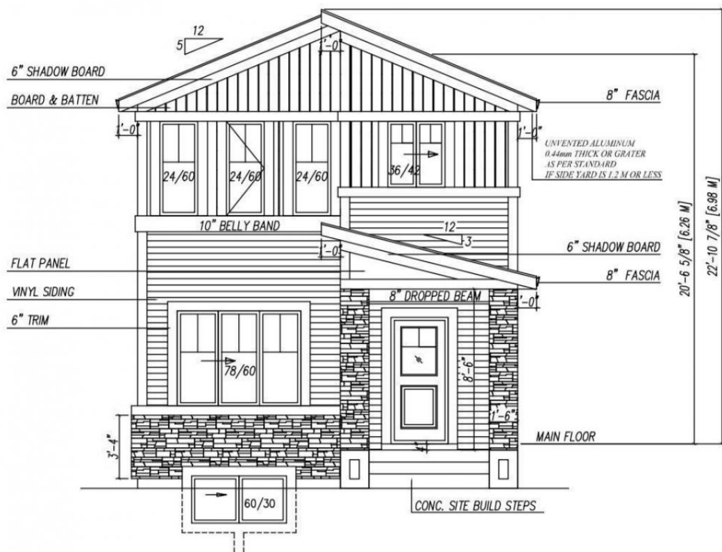
FRONT ELEVATION
