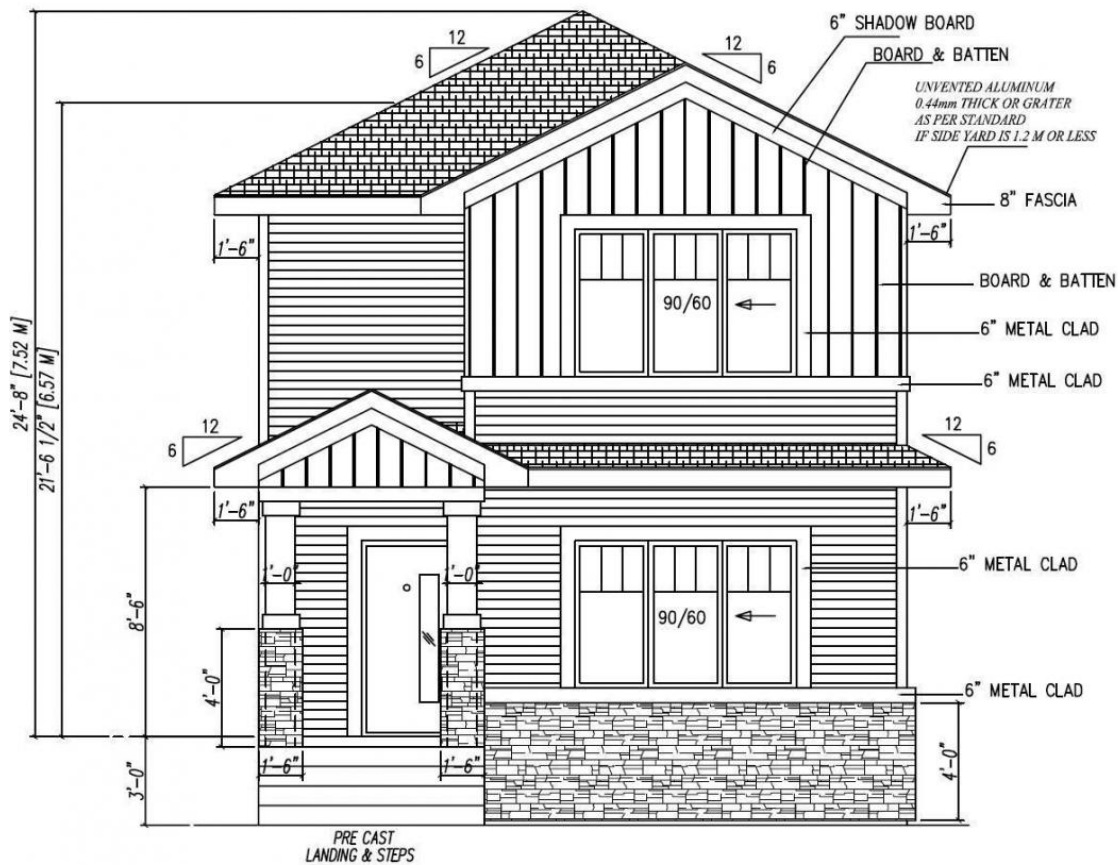
FRONT ELEVATION STONE 118 SQ.FT.
