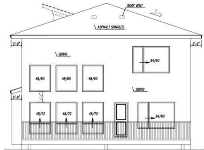
REAR ELEVATION
