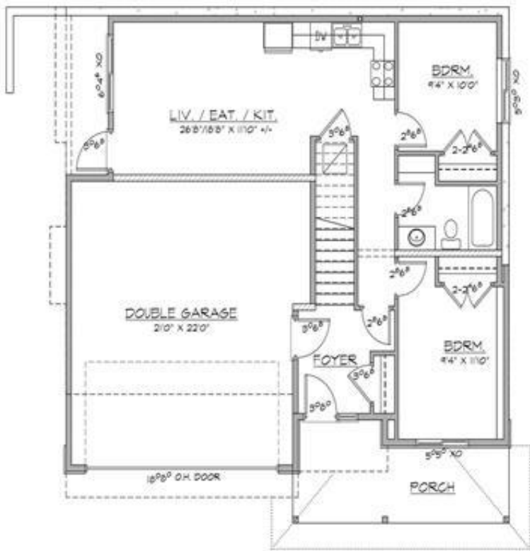
LOWER FLOOR PLAN 900 SQ. FT. (2 BDRM SUITE 760 SQ. FT.)
