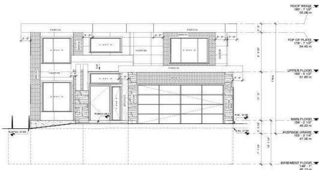
1 Front Elevation
