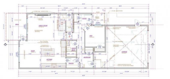
MAIN FLOOR AREA 2,127 sq. ft.
