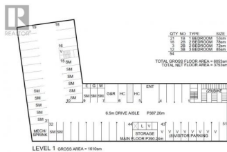
LEVEL 1 GROSS AREA = 693.0sqm
