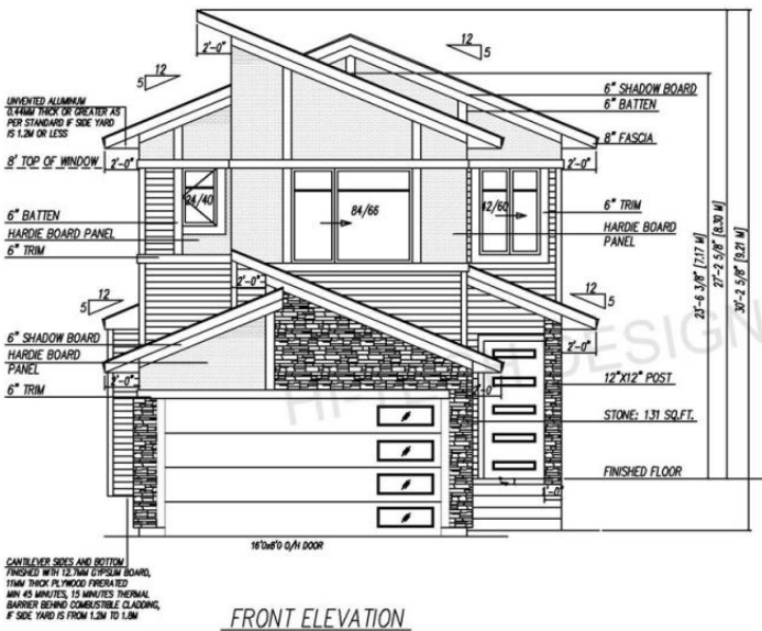
FRONT ELEVATION
