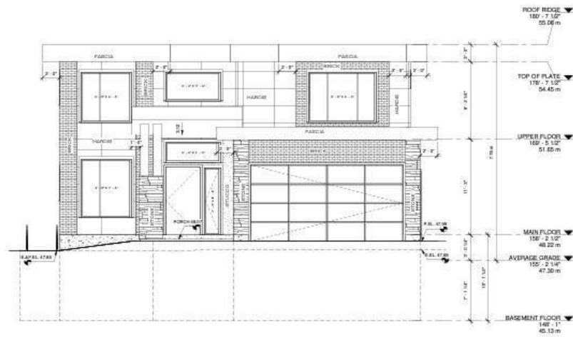
1. Front Elevation 1/4" = 1'-0"
